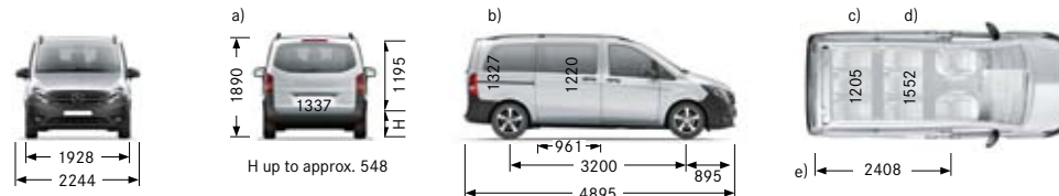
Compact Vito Tourer with 3200 mm wheelbase
