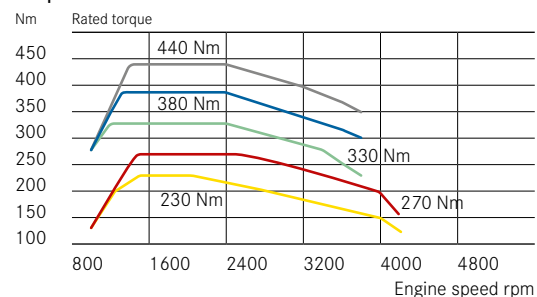
Torque curves:
